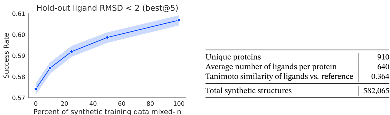
Figure 6. PEARL’s performance scales with the addition of synthetic data. The plot (left) shows a monotonic improvement in success rate (best@5, RMSD < 2 Å) for a smaller variant of PEARL on a fixed hold-out set as the proportion of synthetic data increases. The table (right) summarizes the scaling experiment’s dataset, which included 582,065 synthetic structures across 910 proteins. A larger synthetic dataset was used to train the flagship PEARL model.
