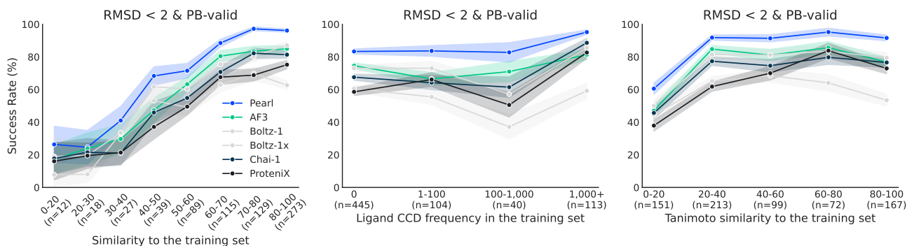
Figure 4. Stratified analysis of PEARL’s generalization on the RnP in the unconditional cofolding mode. Shown are the best@5 success rate for generating valid poses (RMSD < 2 Å and PB-valid) when stratified by (left) overall similarity to the training set (product of binding pocket coverage and combined overlap score [SuCOS] of the ligand pose [23]), (middle) ligand frequency, and (right) Tanimoto similarity. PEARL exhibits strong generalization in the most challenging, low-similarity regimes, where it generally leads other models. The number of test examples in each slice is denoted by n . Boltz-2 is excluded as its expanded training set does not conform to the same similarity measures.
