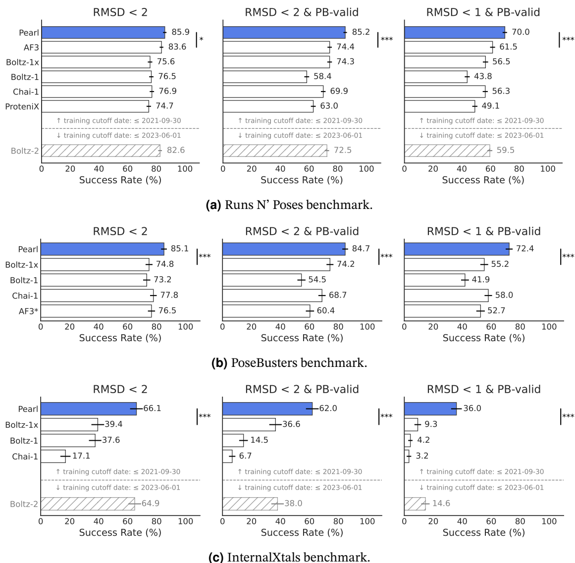
Figure 3. PEARL demonstrates state-of-the-art performance in the unconditional cofolding mode across multiple benchmarks. Shown are best@5 success rates for generating accurate (RMSD < 1 Å and < 2 Å) and physically valid (PB-valid) poses. Dashed lines group models for fair comparison (e.g., based on the training cutoff dates). Note 1(*): AlphaFold 3 results for PoseBusters use officially released metrics for poses selected for max confidence out of 25 samples (not best@5). Note 2: AlphaFold 3 was excluded from the InternalXtals benchmark due to license restrictions. Note 3: Trained with additional public data up to 2023-06-01, Boltz-2 is not directly comparable to the other evaluated models, which use 2021-09-30 or earlier training cutoff. Note 4: Statistical significance (one-sided t-test) is shown as: *: p \leq 0.05 , **: p \leq 0.01 , ***: p \leq 0.001 .
