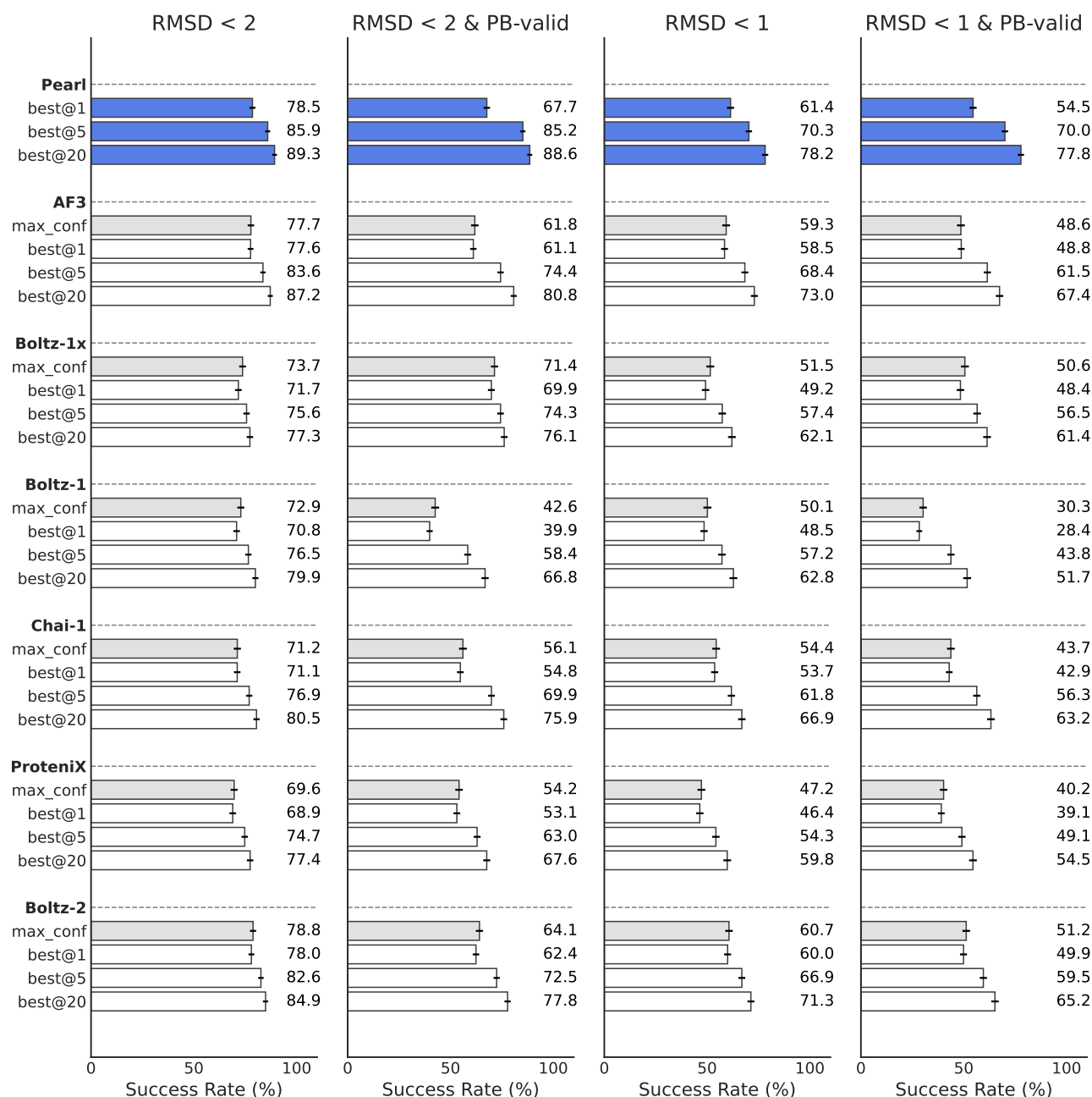
Figure 11. Comparison of the success rates for the best@1, best@5, and best@20 poses versus poses selected with a confidence model (out of 20 sampled) for each of the models on the Runs N' Poses benchmark. The differences between max confidence and randomly selected (best@1) poses are not statistically significant for any of the models. In many cases, PEARL's best@1 pose ( i.e. , a single random pose) outperforms max confidence poses produced by other models.
