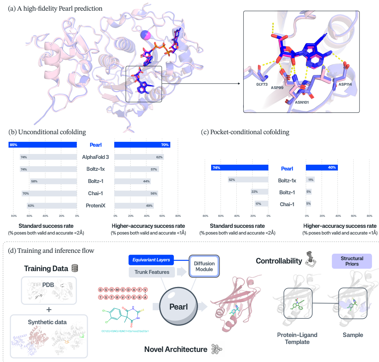
Figure 1. (a) PEARL prediction (magenta) superimposed on the experimental ground truth (blue) for SARS-CoV-2 (PDB: 8S8X, in the Runs N' Poses, released March 2024); PEARL performance in the (b) unconditional (Runs N' Poses) and (c) pocket-conditional (InternalXtals) cofolding modes; (d) PEARL training and inference flow.
