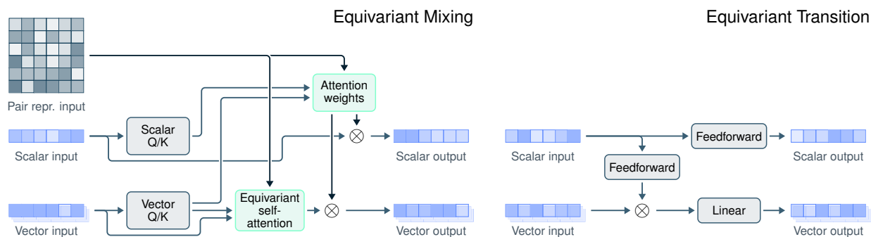
Figure 2. Key components of the equivariant diffusion module, including the equivariant transformer architecture (left) and the equivariant feed-forward layer with a gated nonlinearity for vector components (right).
