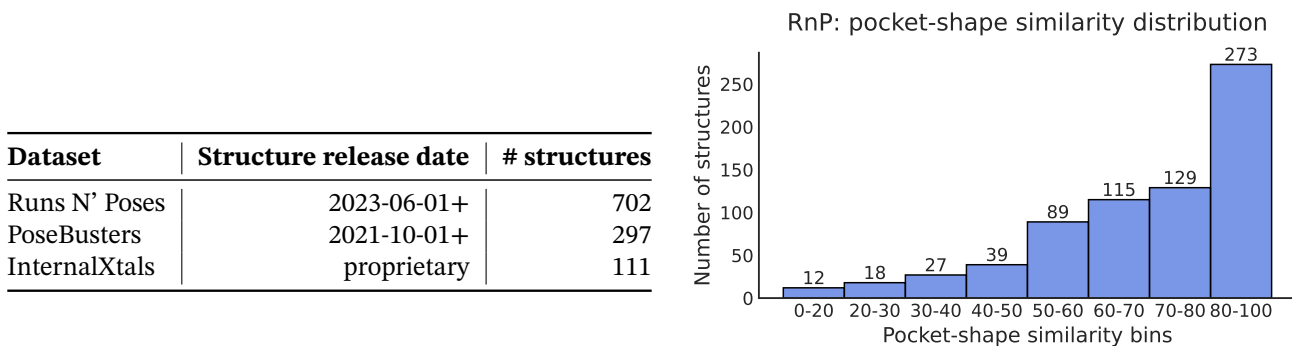
Figure 10. (Left) statistics of the RnP, PoseBusters, and InternalXtals datasets used for analysis and benchmarking. (Right) Histogram of the number of structures in each pocket-shape similarity bin of the RnP dataset.
