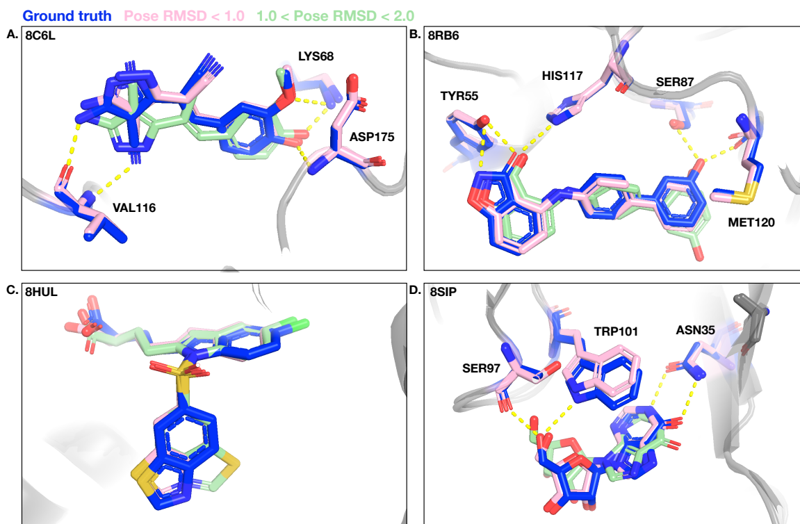
Figure 9. Qualitative analysis of the importance of high-accuracy predictions. The figure compares high-accuracy poses (RMSD < 1 Å, pink) with lower-accuracy poses (1 Å < RMSD < 2 Å, green). The lower-accuracy poses, while under the standard RMSD < 2 Å threshold, exhibit critical errors that limit their utility for drug discovery, such as ring flips (A, B, C) and slight translations (D). (A) A 1.99 Å pose of CK2-TN01 in complex with human protein kinase CK2 alpha displays a ring flip and misses a key interaction, which is correctly formed in the 0.42 Å pose. (B) A 1.70 Å pose of M689 in complex with AKR1C3 displays a problematic ring flip. Shown in comparison to the 0.36 Å pose. (C) A 1.51 Å pose of lanifibranor bound to human PPAR \delta displays an incorrect flip of the thiazole ring. Shown in comparison to a 0.58 Å pose. (D) A 1.54 Å pose of inosine bound to a mouse IgG fragment displays a slight translation, missing all the key interactions that are correctly predicted in the 0.38 Å pose.
