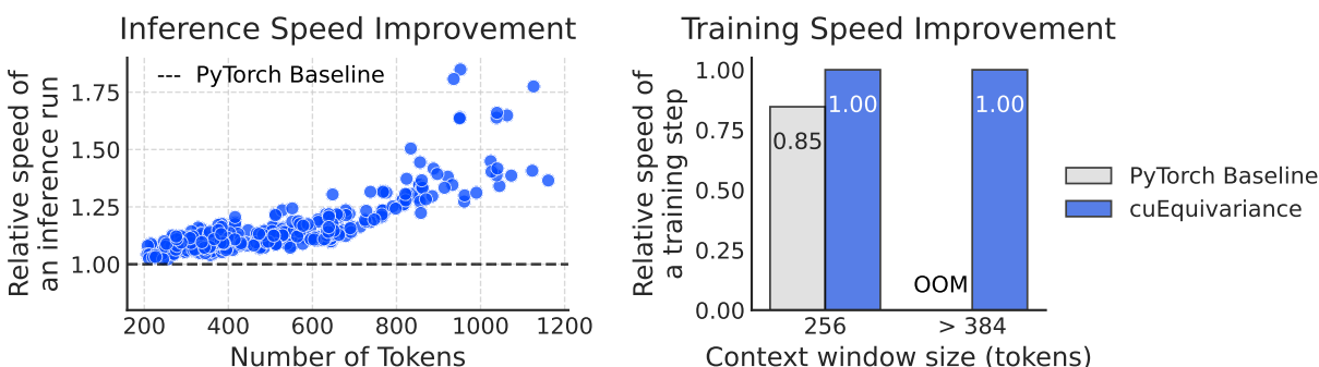
Figure 7. NVIDIA’s optimized cuEquivariance kernels provide significant acceleration for PEARL relative to a vanilla PyTorch baseline. The kernels deliver a 10–80% speedup at inference time (left) and a 15% training speedup (right).
