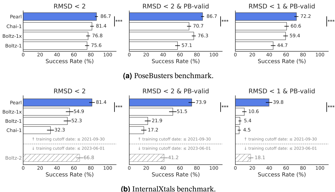
Figure 5. PEARL demonstrates state-of-the-art performance in the conditional cofolding mode across multiple benchmarks. Metrics shown are best@5 (from 20 samples). Dashed lines group models for fair comparison based on the training cutoff dates. Note 1: AlphaFold 3 was excluded due to license restrictions. Note 2: Trained with data up to 2023-06-01, Boltz-2 is not directly comparable to models using earlier cutoffs.
